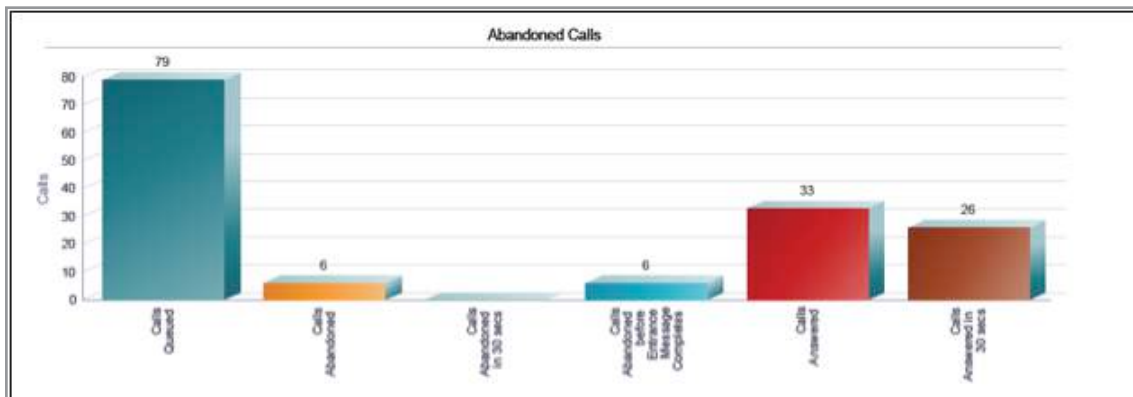
Figure 55 Abandoned Call Report – Abandoned Calls Bar Chart
